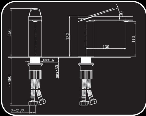
Lavabo Basin Mixer
