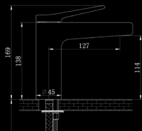
Lavabo Basin Mixer
